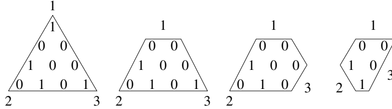
Figure 3: Payoffs of a particular player in a self-anonymous game with n = 3 and k = 3 . Initially all actions are pairwise undominated. If one of the other players eliminates action 1, action 3 weakly dominates action 1. Action 1 then becomes undominated if some player deletes action 3, and dominated by action 2 if one more player deletes action 3, and some player deletes action 2.
