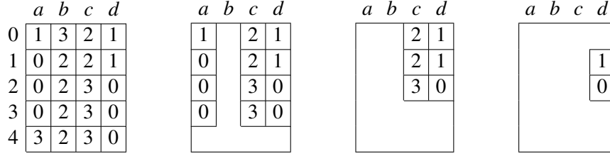
Figure 1: A matrix and a sequence of eliminations
