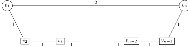
Fig. 1: An example where DAA leads to an approximation ratio of (n - 1)/2
