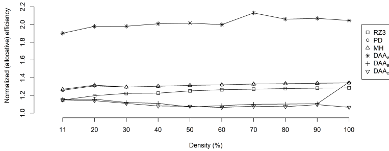
Fig. 2: Average efficiency over all instances
