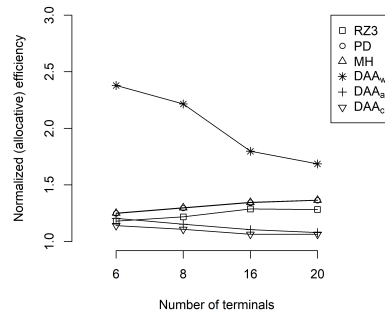
Fig. 3: Average efficiency depending on number of terminals
