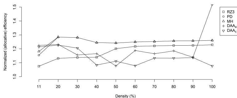
Fig. 4: Efficiency for 6 terminals
