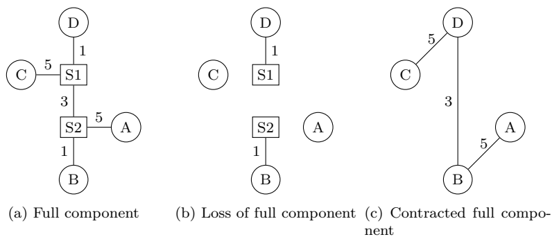
Fig. 7: Full components
