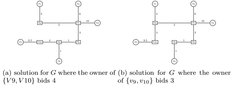
Fig. 11: MST-based solutions
