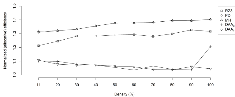
Fig. 5: Efficiency for 20 terminals
